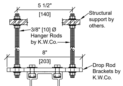
Optional Drop Rod Bracket Mount
