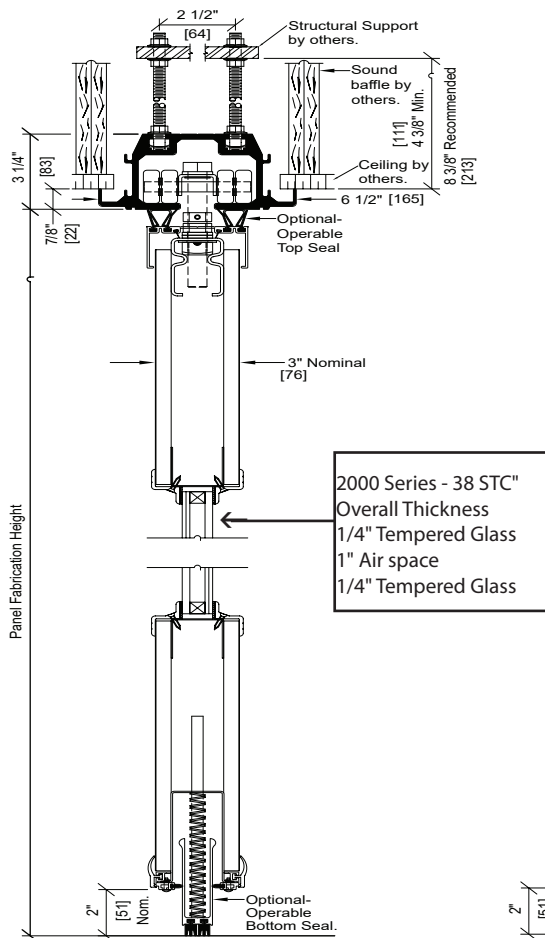
850 Hinged Pairs Aluminum Track and Carrier
