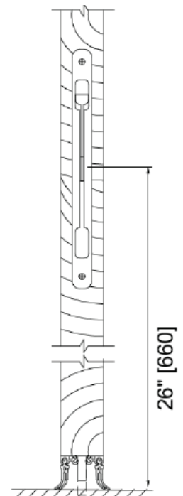
Edge-Activated Mortise Footbolt Pin
